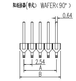
安装尺寸 MOUNTING MEASUREMENT
